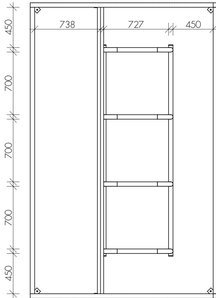
SIDE ELEVATION
